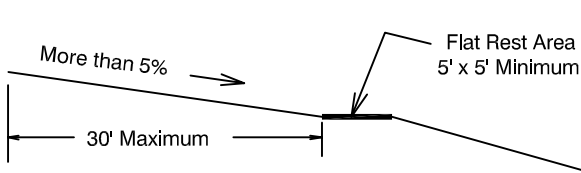
Sidewalk Profile
