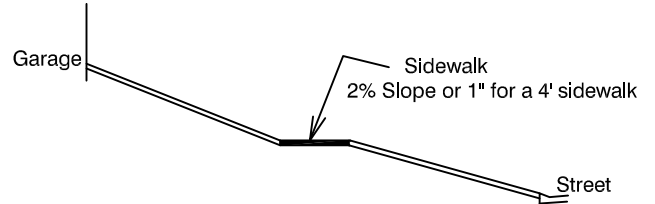
Driveway Profile
