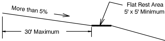
Sidewalk Profile
