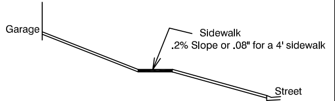
Driveway Profile
