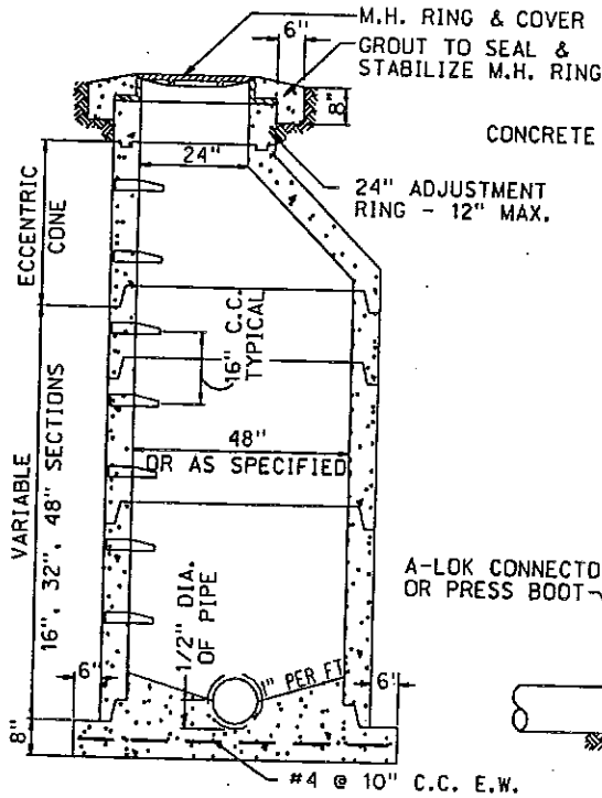
MANHOLE SECTIONAL ELEVATION
