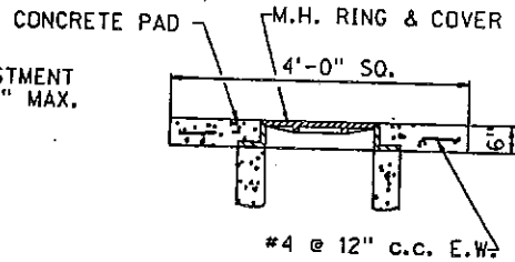
SURFACE MANHOLE RING & COVER INSTALLATION
